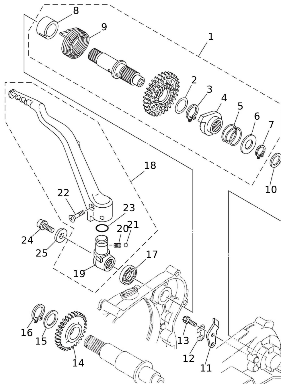
Starter
