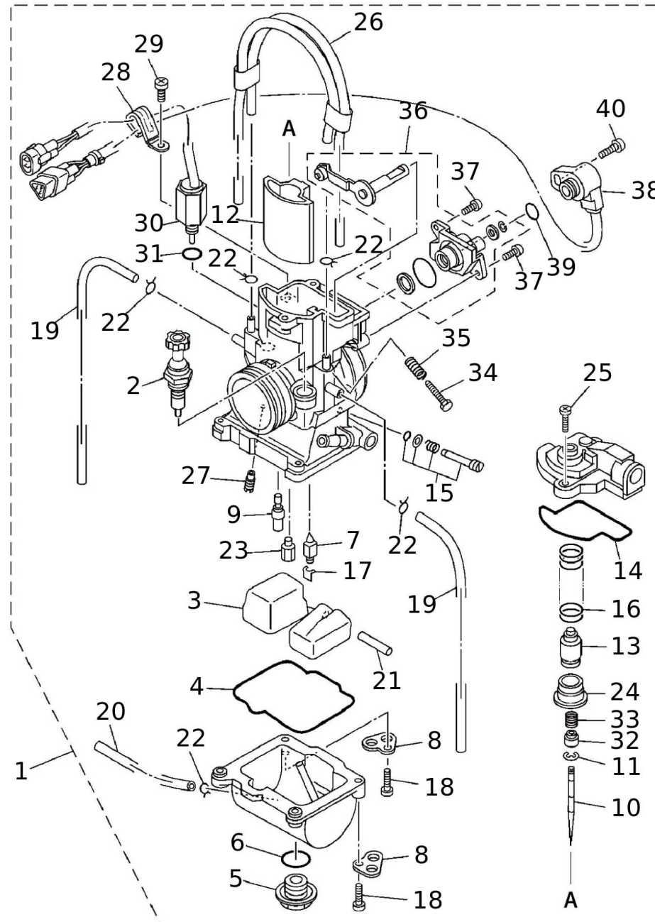
CARBURETOR ASSY 1
