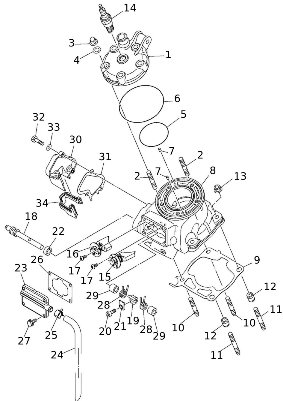
Head - Cylinder
