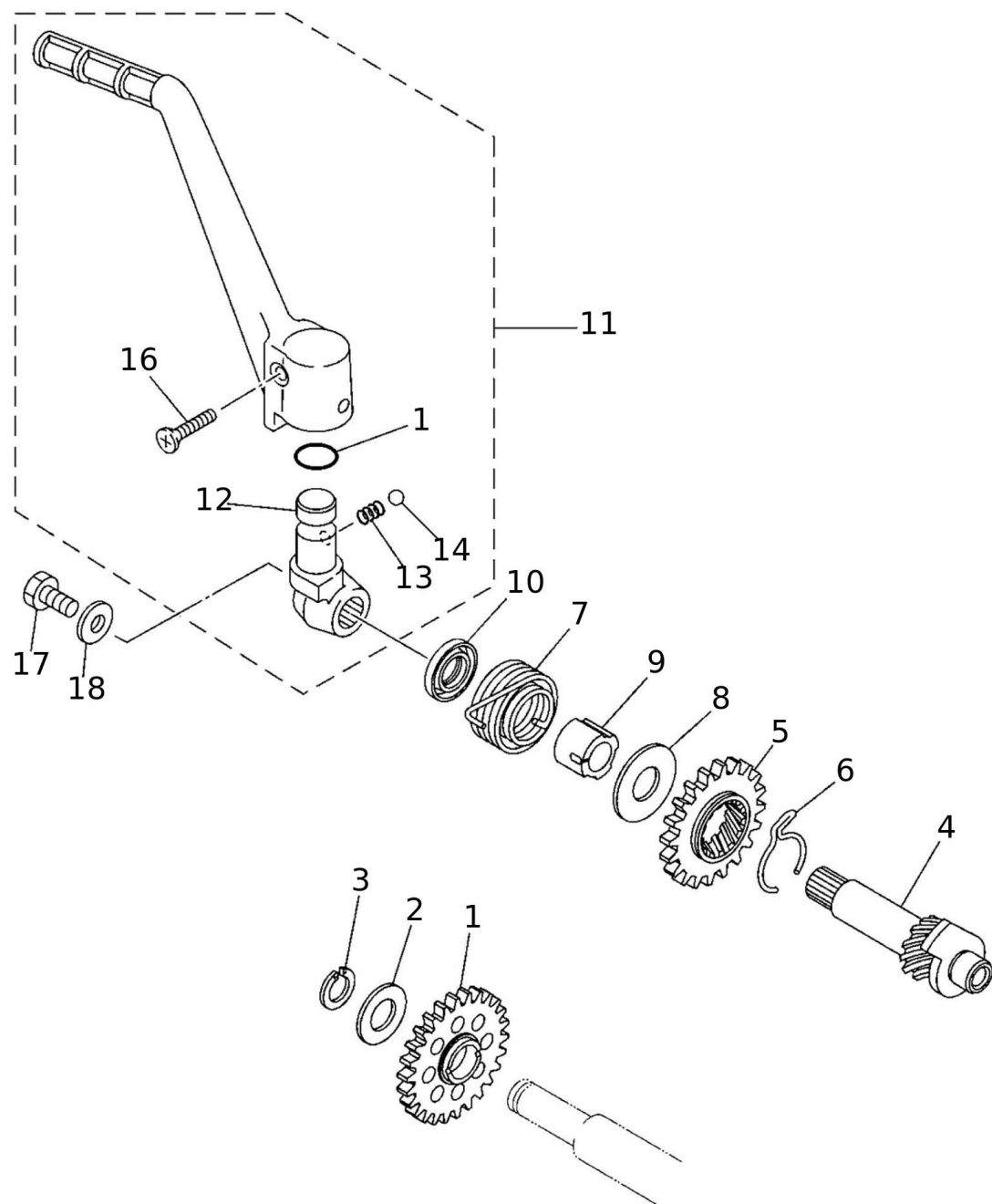
Starter
