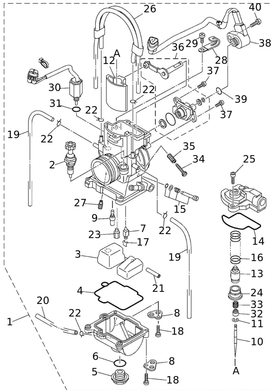
CARBURETOR ASSY 1
