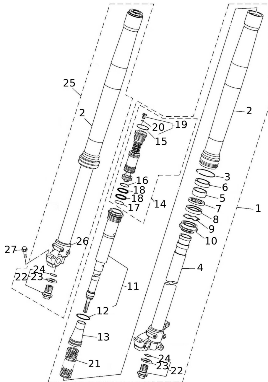
Fork
