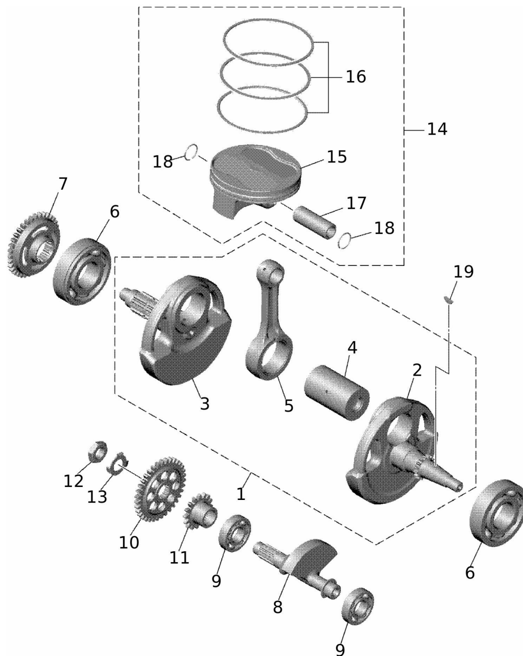
Crankshaft
