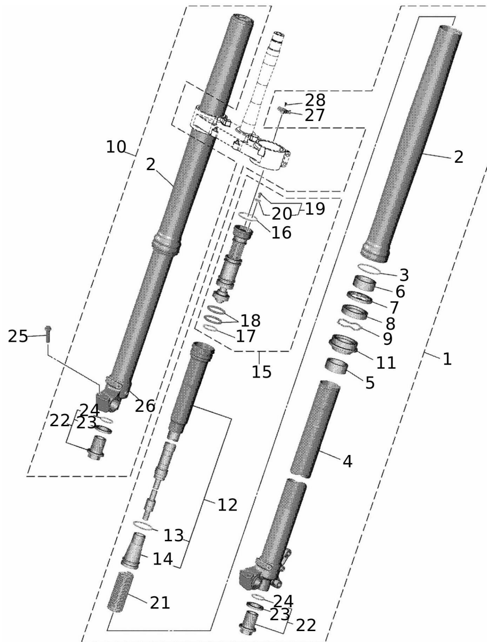
Fork
