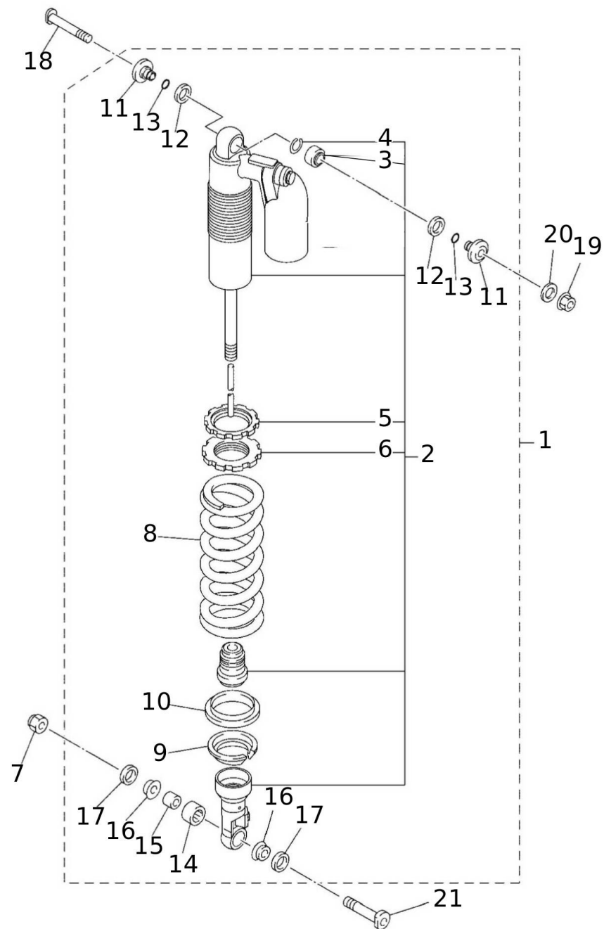
3 - Rear absorber
